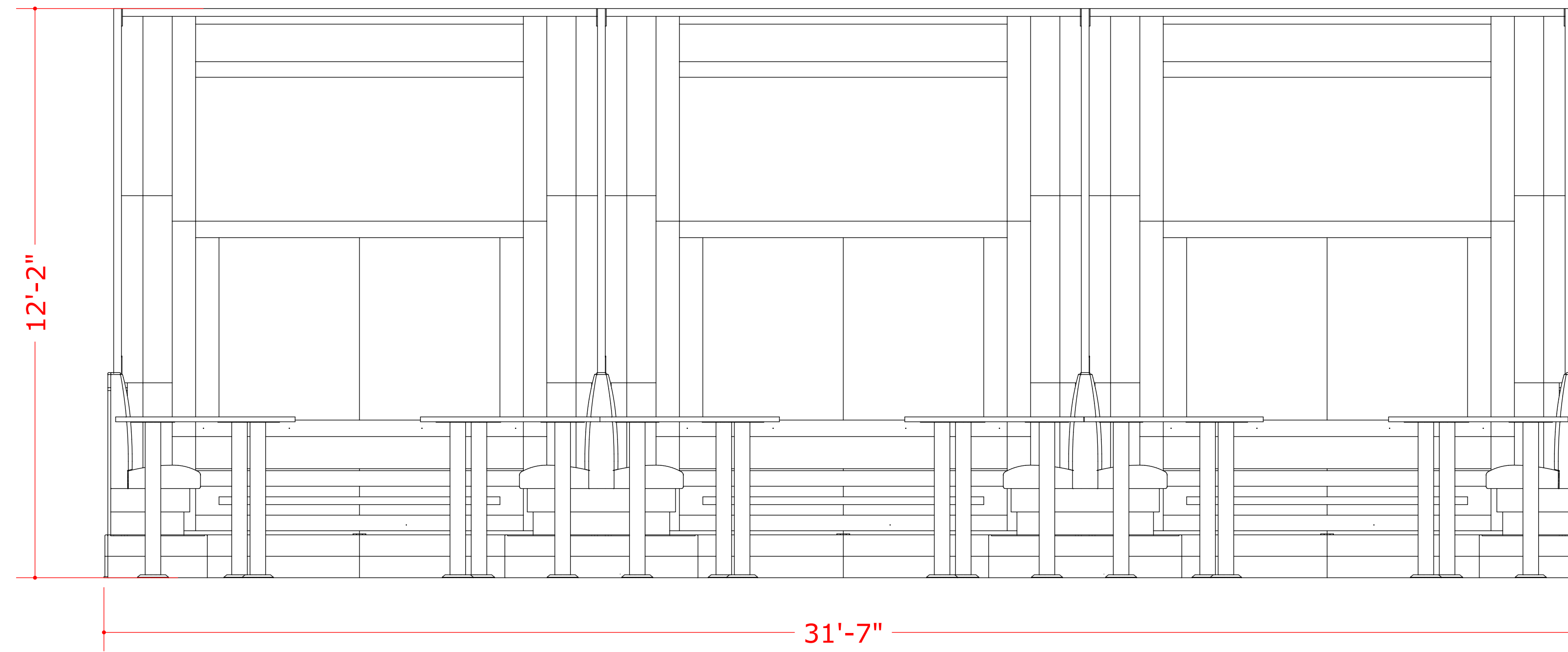
ELEVATION D SCALE 1/2"=1'-0"
