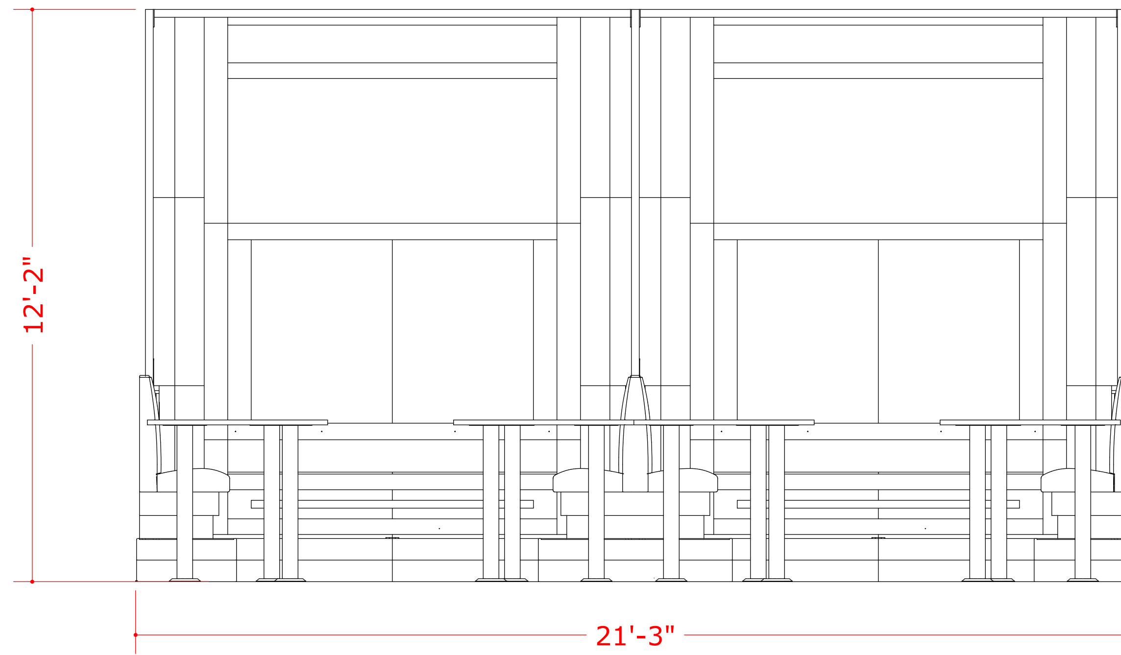
ELEVATION D SCALE 1/2"=1'-0"
