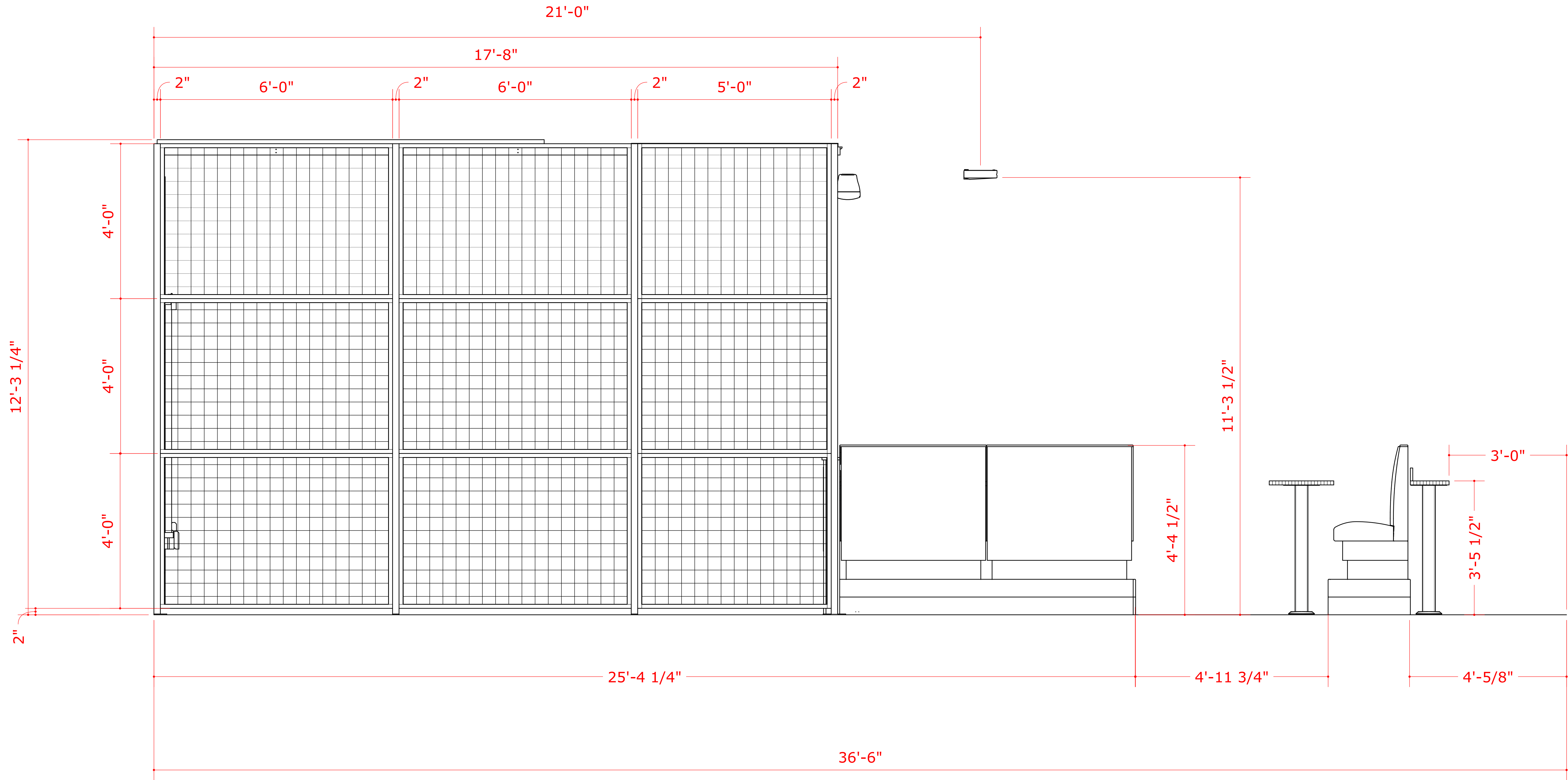
ELEVATION A SCALE 3/4"=1'-0"
